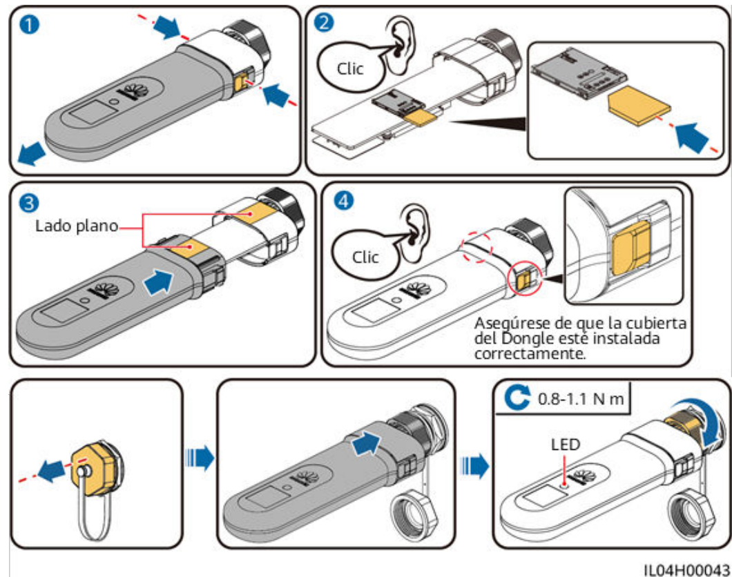
Figura 5-37 Smart Dongle 4G: SDongleB-06
